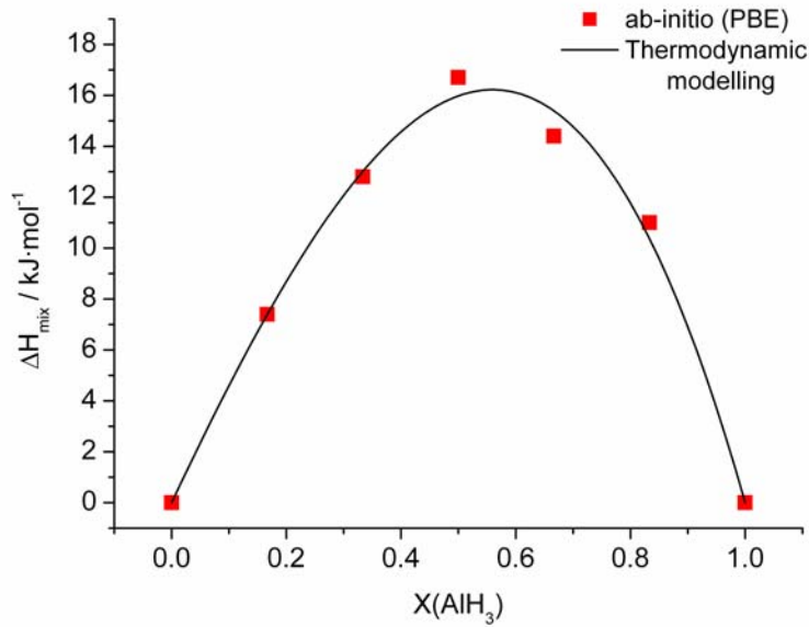
Figure 3: Calculated enthalpy of mixing in the trigonal solid solution at 298 K and 1bar in comparison with the results from first-principles calculations
