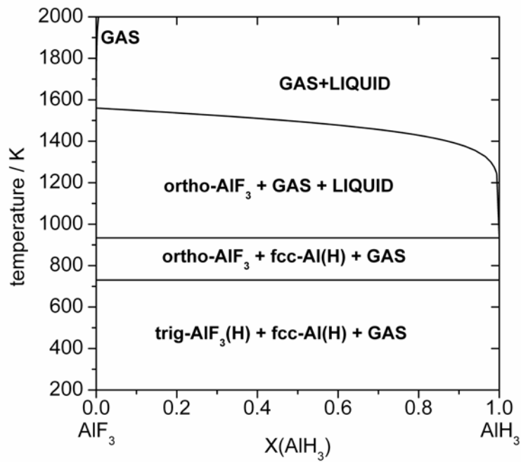
Figure 4: AlH 3 -AlF 3 pseudo-binary phase diagram
