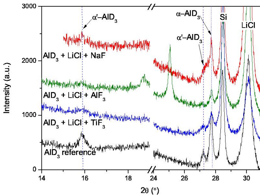
Figure 2: AID 3 cryo milled with NaF (sample 7), AlF 3 (sample 8) or TiF 3 (sample 9) for 10 min. No change in peak positions of AID 3 is seen. The label Si corresponds to the Bragg peaks for the Si standard.
